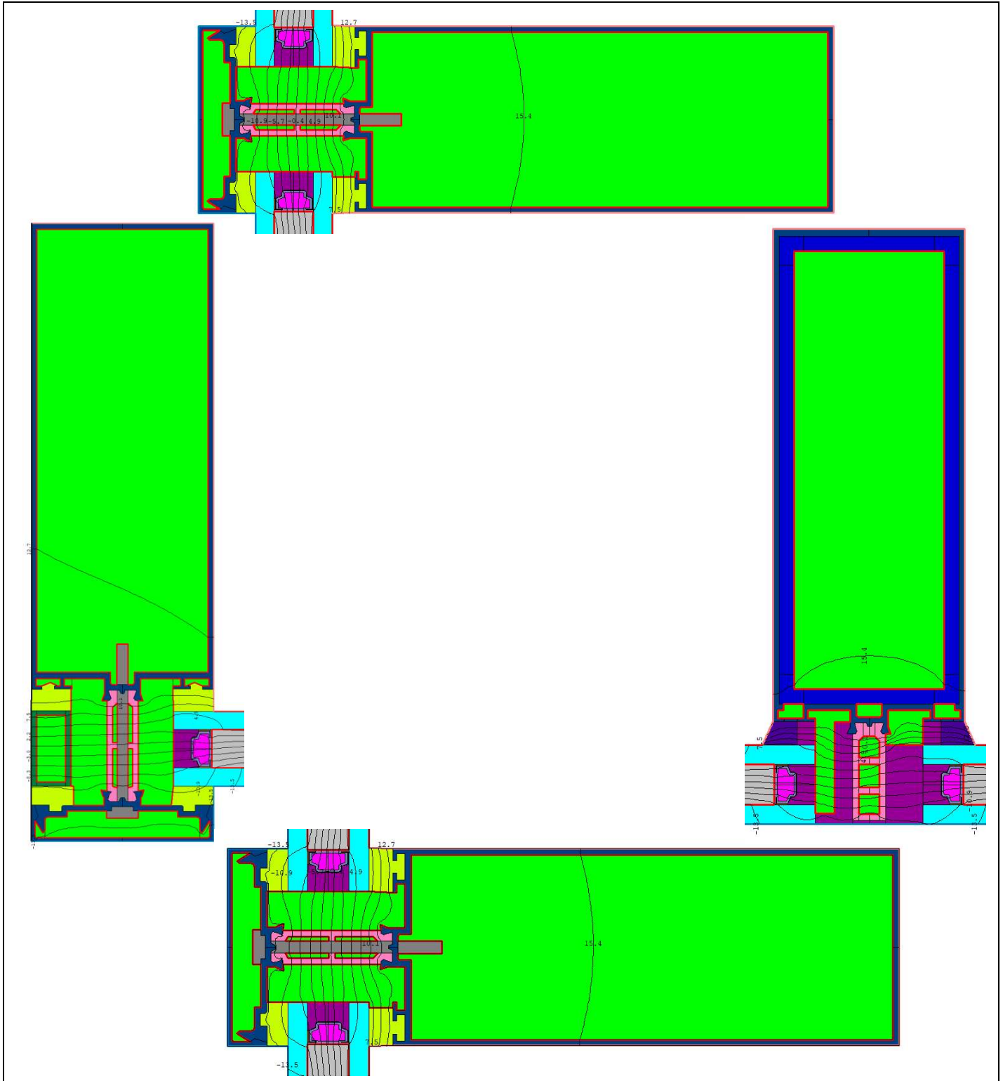
Figure 1: Thermal Modelling Result of the most dominant frame type (Curtain Wall)
